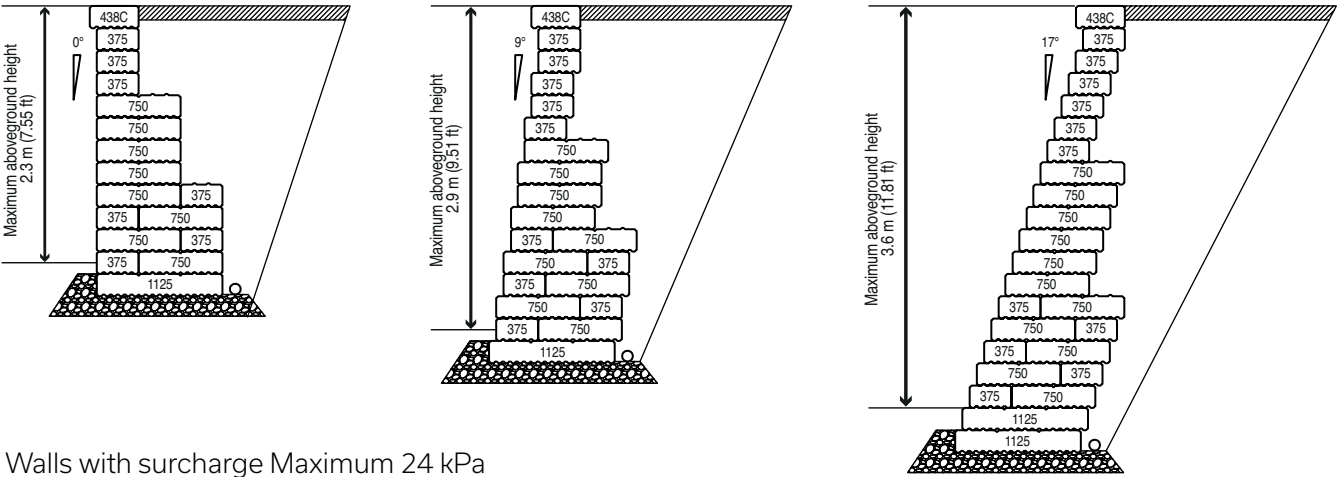
Walls with surcharge Maximum 24 kPa
