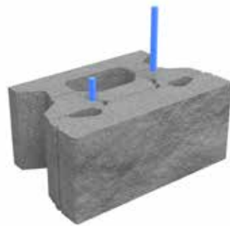
Insert connecting pin into pin holes
