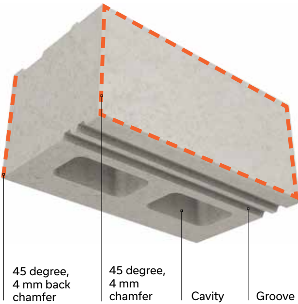
180 mm medium underside unit
