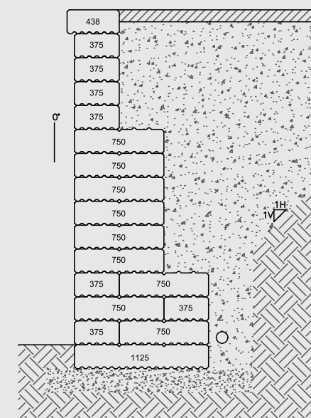
Grande Smooth Wall 3 m (9.8 ft.) 15 rows straight gravity
