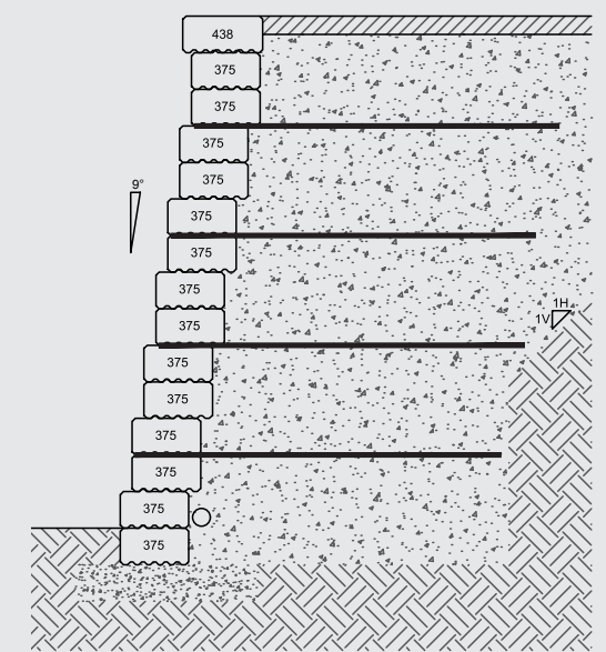
Grande Smooth Wall 3 m (9.8 ft.) 15 rows 9° reinforced slope
