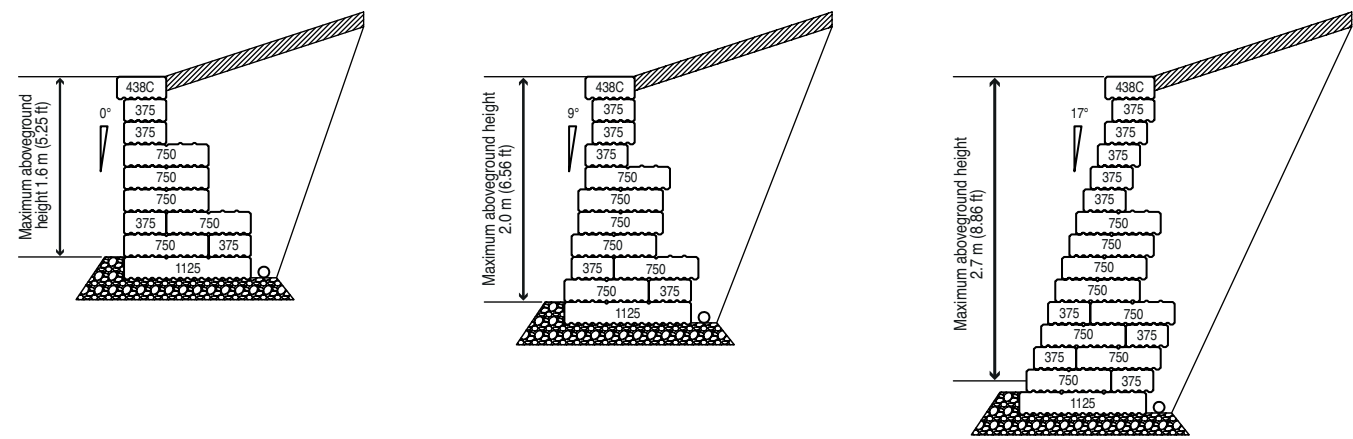
Walls with surcharge at varying angles (maximum gradient of slope—1 vertical: 3 horizontal)
