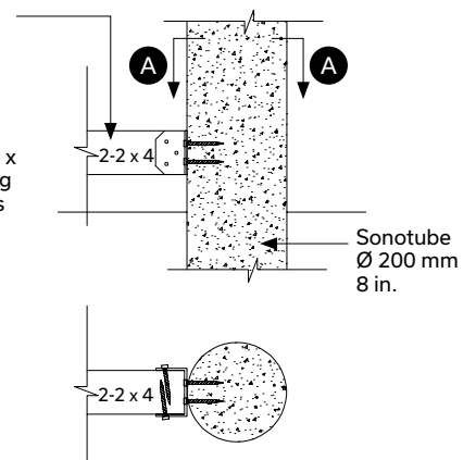
CROSS-SECTION A-A
