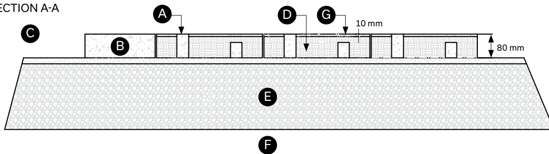
CROSS-SECTION A-A
