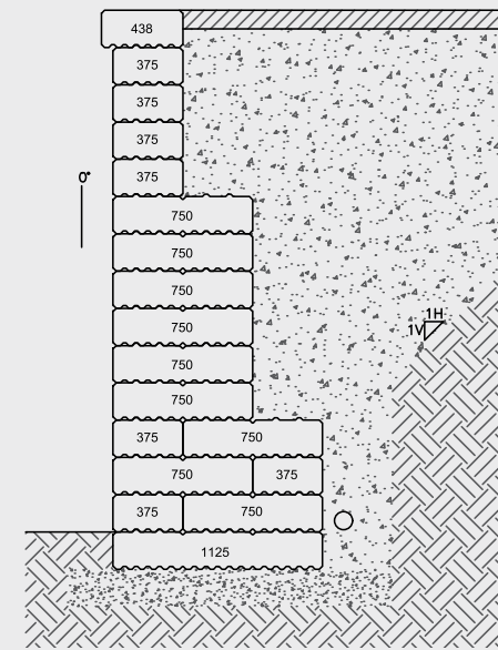
Grande Smooth Wall 3 m (9.8 ft.) 15 rows straight gravity
