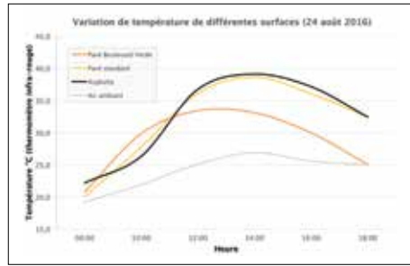
Daily surface temperatures of different pavements.
