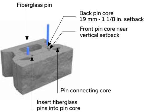
WALL UNIT TO WALL UNIT CONNECTION
