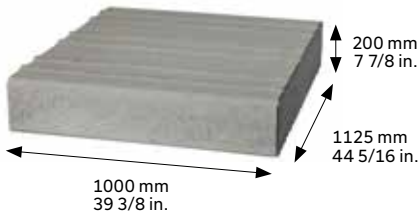
1125 STANDARD
