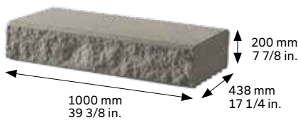
CAPPING 438
