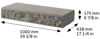
STEP 175
