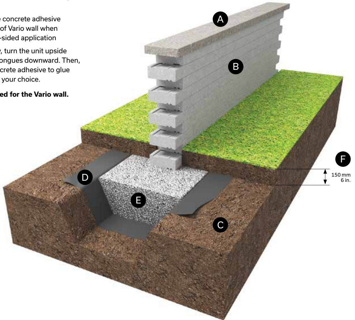
ISOMETRIC VIEW
