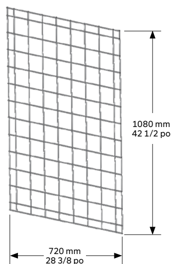
POSE VERTICALE
